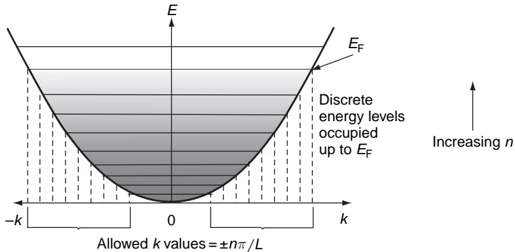
Figure 1.7 Schematic version of the parabolic relationship between the allowed electron wave vectors and the their energy for electrons confined to a one-dimensional potential well. Shaded energy regions represent those occupied with electrons
