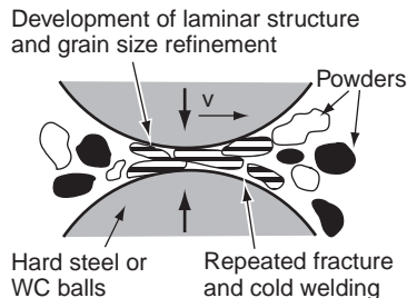
Figure 1.20 Schematic representation of the mechanical alloying process
