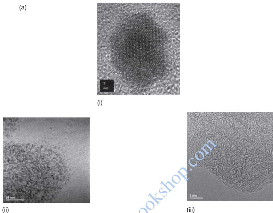
Figure 1.1 Classification of nanostructures (a) Nanoparticles and nanopores (nanosized in three dimensions): (i) high-resolution TEM image of magnetic iron oxide nanoparticle, (ii) TEM image of ferritin nanoparticles in a liver biopsy specimen, and (iii) high-resolution TEM image of nanoporosity in an activated carbon. (b) Nanotubes and nanofilaments (nanosized in two dimensions): (i) TEM image of single-walled carbon nanotubes prepared by chemical vapour deposition, (ii) TEM image of ordered block copolymer film, and (iii) SEM image of silica nanotube formed via templating on a tartaric acid crystal. (c) Nanolayers and nanofilms (nanosized in one dimension): (i) TEM image of a ferroelectric thin film on an electrode, (ii) TEM image of cementite (carbide) layers in a carbon steel, and (iii) high-resolution TEM image of glassy grain boundary film in an alumina polycrystal. Images courtesy of Andy Brown, Zabeada Aslam, Sarah Pan, Manoch Naksata and John Harrington, IMR, Leeds
