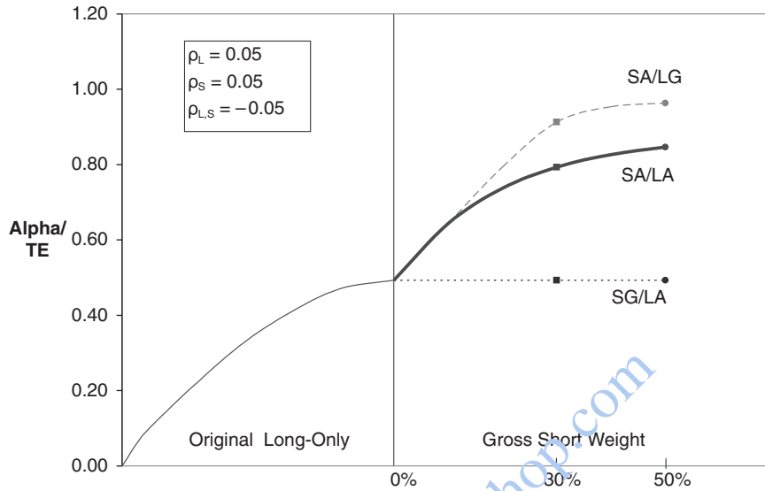
EXHIBIT 1.10 Alpha/TE versus Short Weight: Generics on the Short and/or Long Sides Source: Morgan Stanley Research
