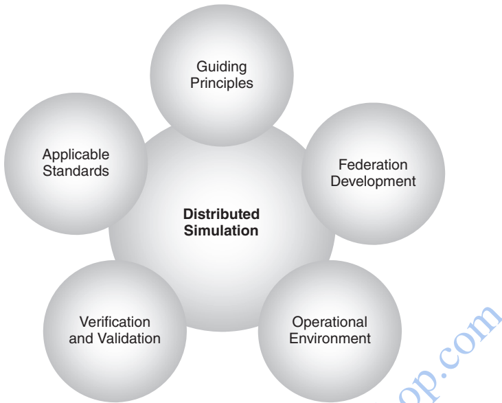
Figure 1.3 Distributed simulation.
