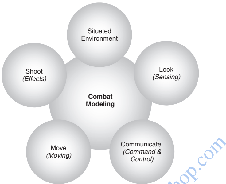
Figure 1.2 Combat modeling.
